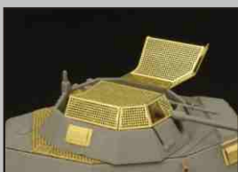
HLX48249 Sd.Kfz.222 GRILLS PE parts for ICM kit
