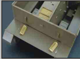
HLX48043 British u. carrier GRILLS photoetched parts for Tamiya kit
